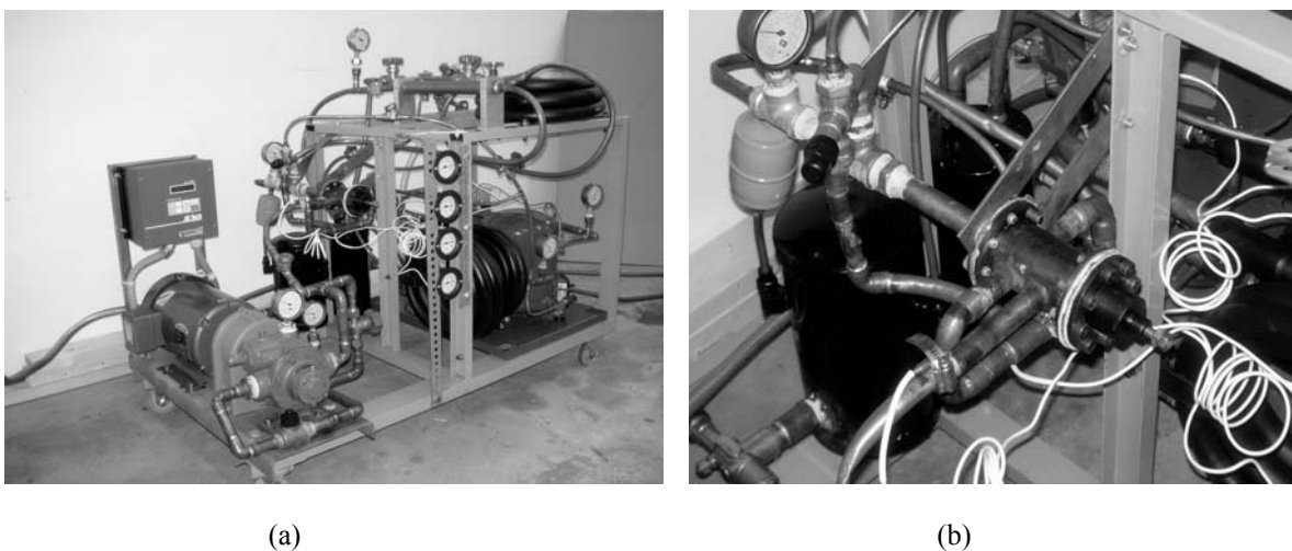
Figure 4. (a) Overall view of the laboratory stand, and (b) Closer view of the ejector device
