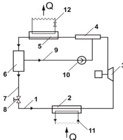
Figure 2. Schematic of the refrigeration system with the condensing ejector as a second-stage compressor
