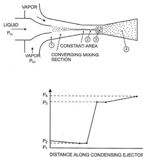
Figure 1. Principle of condensing ejector
