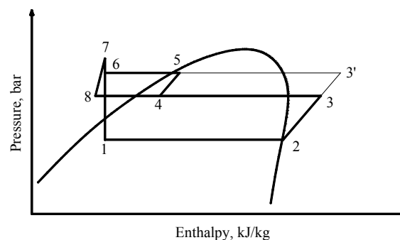
Figure 3. Comparison of p-h diagrams of the new refrigeration cycle with a two-phase ejector, Cycle 1 (points: 1-2-3-4-5-6-1 and 6-7-8-4) and the traditional cycle Cycle 2 (the point: 1-2-3'-6-1).
